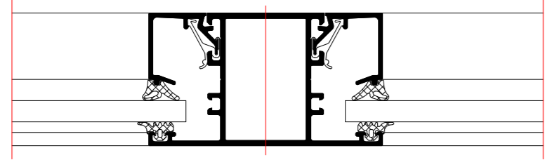
Riegel / Pfosten Transom/mullion
