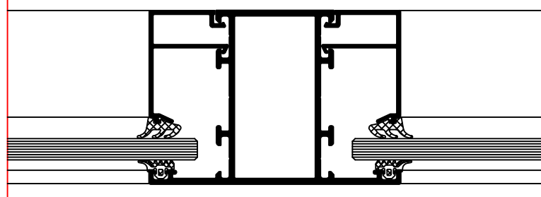
Riegel / Pfosten Transom/mullion
