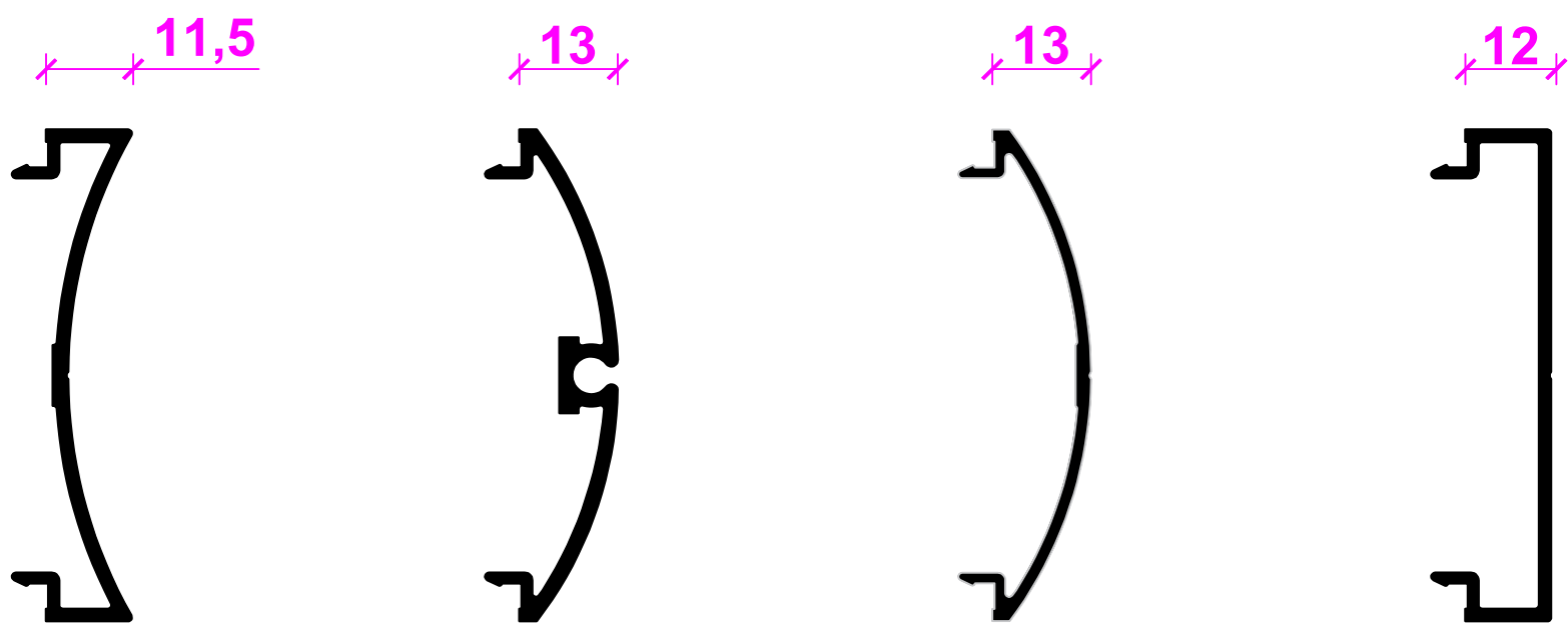
Pendelstulpprofil Swing door meeting stile profile
