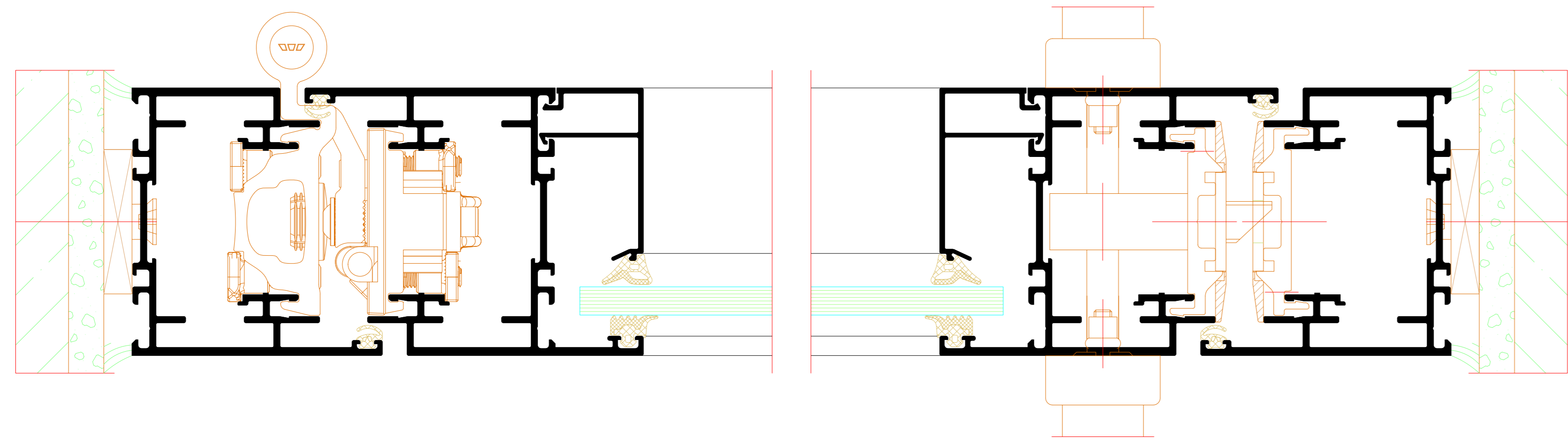
Zweiflügelige Tür Double-leaf door
